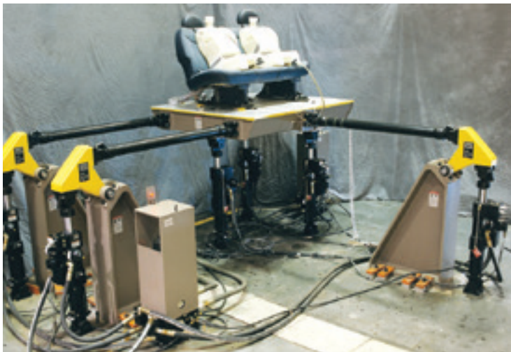
Model 323 Orthogonal MAST System
