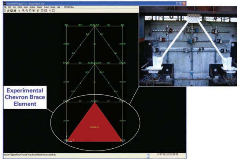
Depiction of the Experimental Element Concept (Schellenberg)
