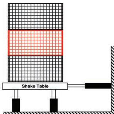
Typical Seismic Simulator Physical Test (Reinhorn)
