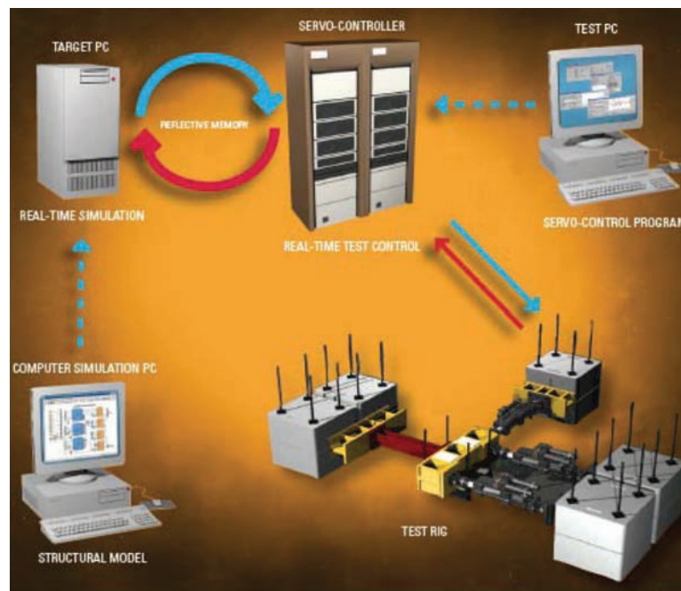
Real-time Hybrid Simulation System Diagram
