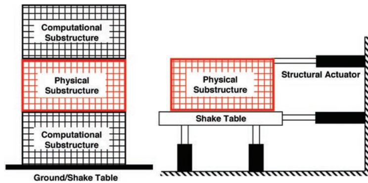
Hybrid Simulation Example (Reinhorn)
