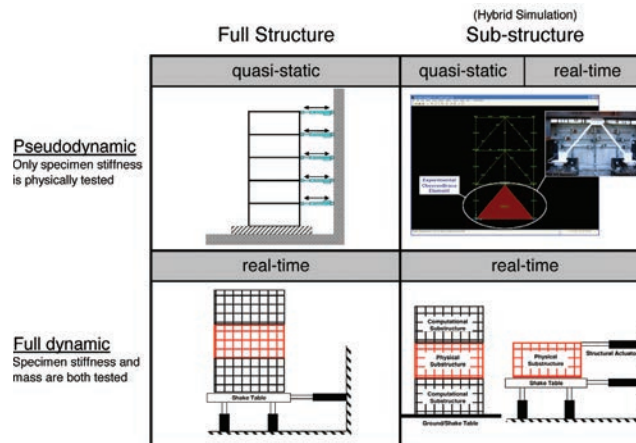
Comparison of Conventional and Hybrid Simulation Testing Techniques
