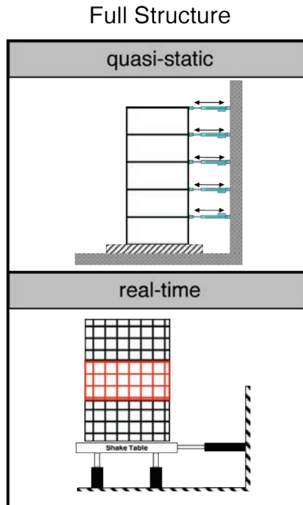
Comparison of Conventional Testing Techniques
